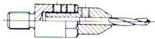
Example of pilot drill w/adapter in standard drill chuck
